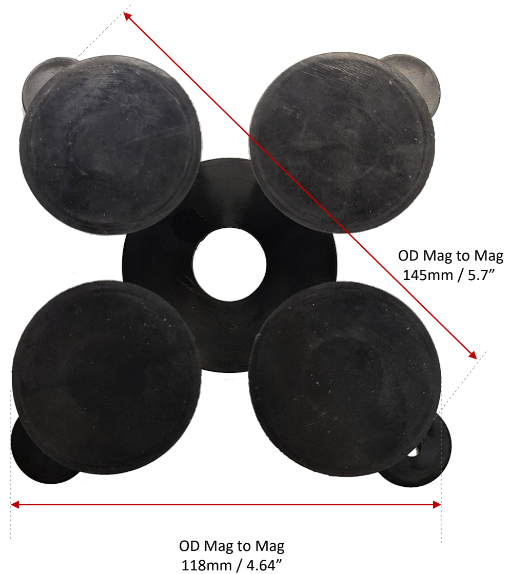
Bottom View
